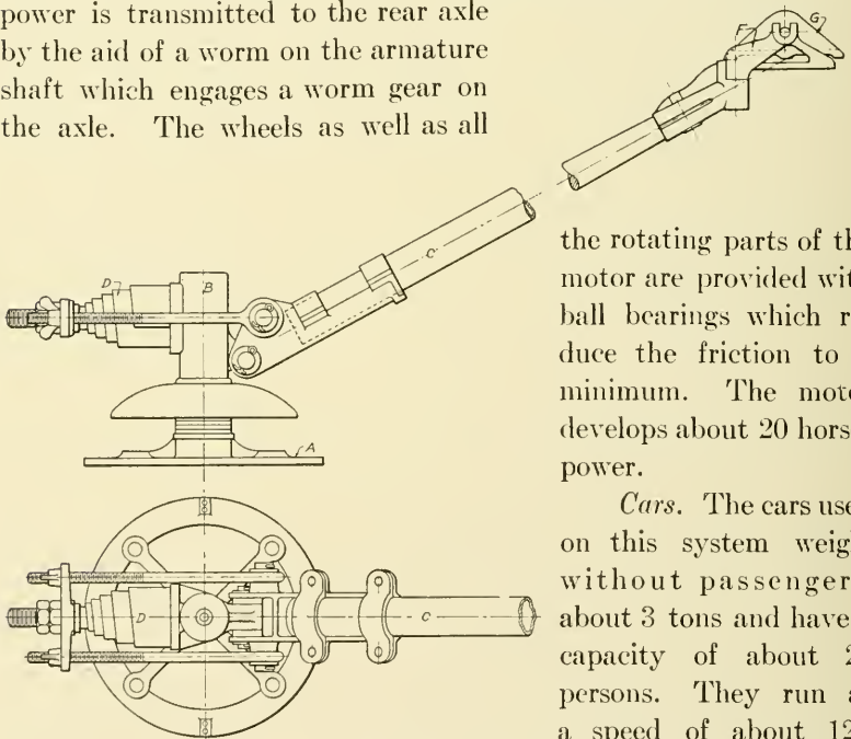
Fig. 2. Detailed Diagrams Showing Trolley Pole and Collector Device
